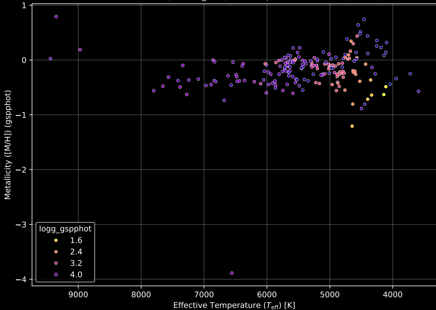
APOGEE DR17 Field: [178+26_MGA] Stellar Population Parameters (n= 203)
