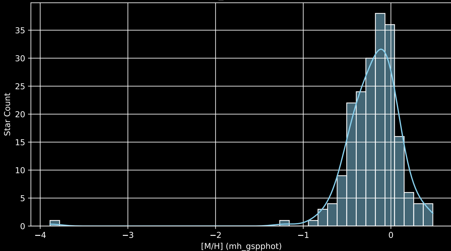
APOGEE DR17 Field: [178+26_MGA [M/H] (mh_gspphot) (n= 199)
