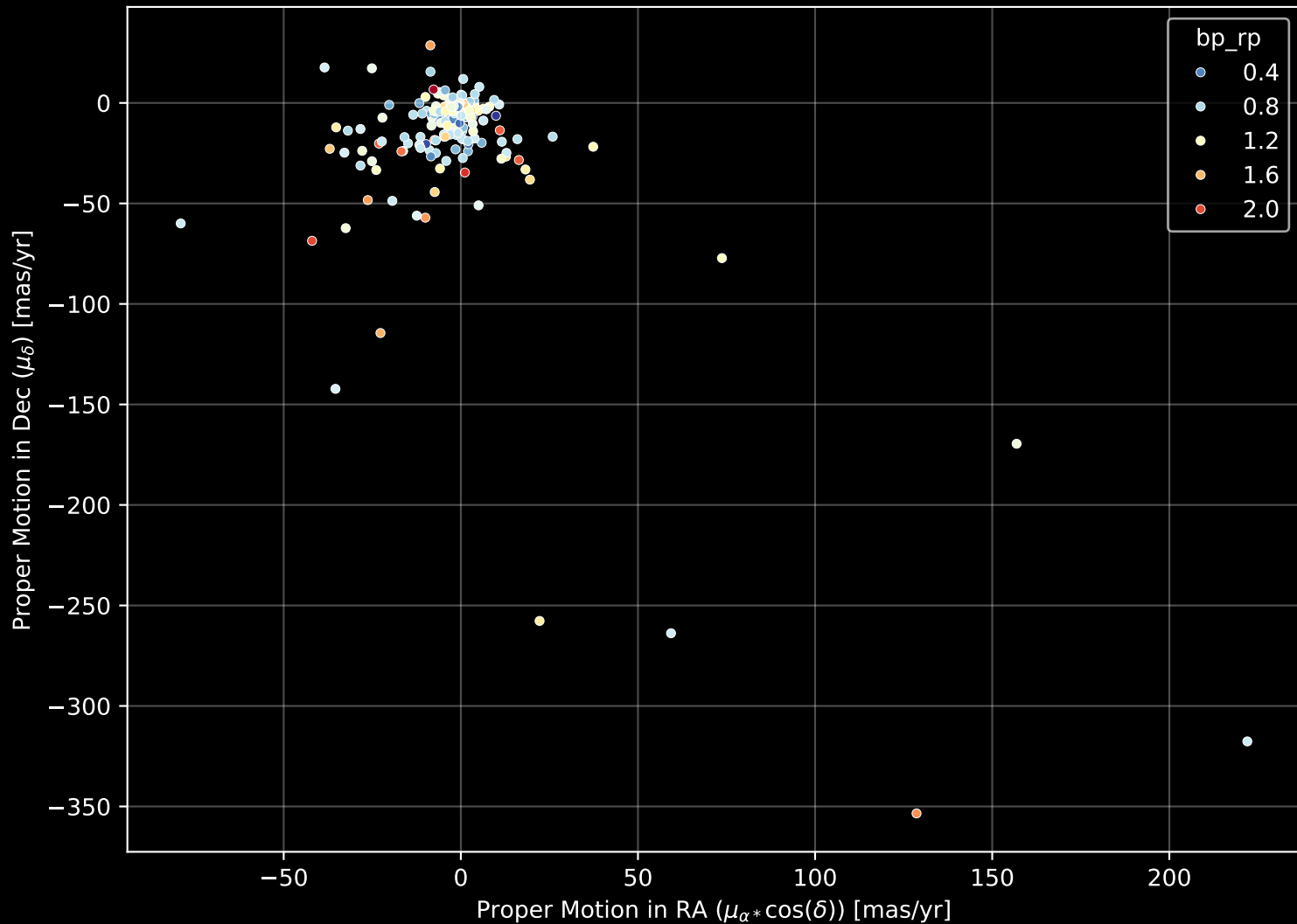
APOGEE DR17 Field: [178+26_MGA] Proper Motion Diagram (n= 203)
