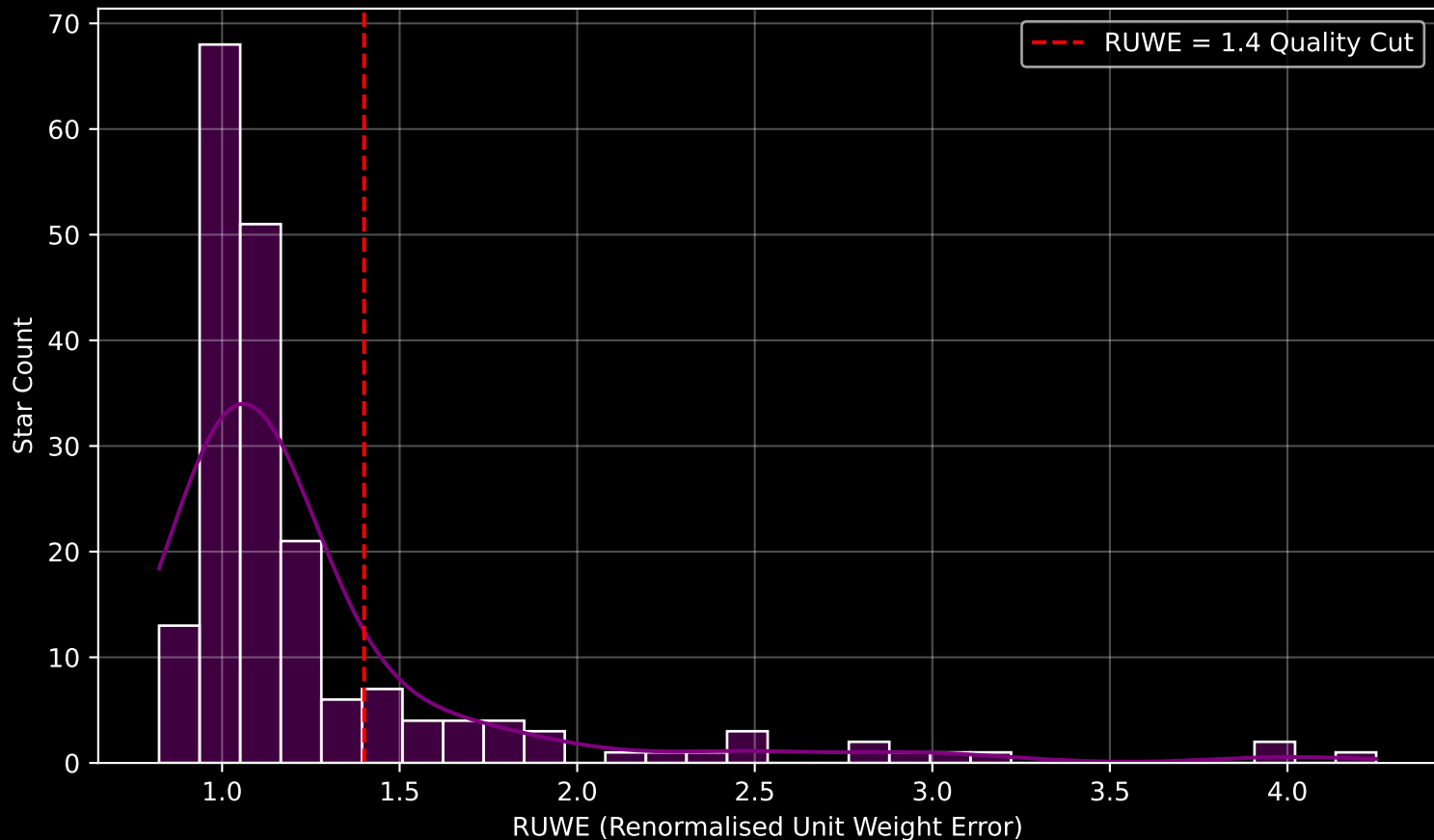
GAPOGEE DR17 Field [178+26_MGA] RUWE Distribution (n= 195)
