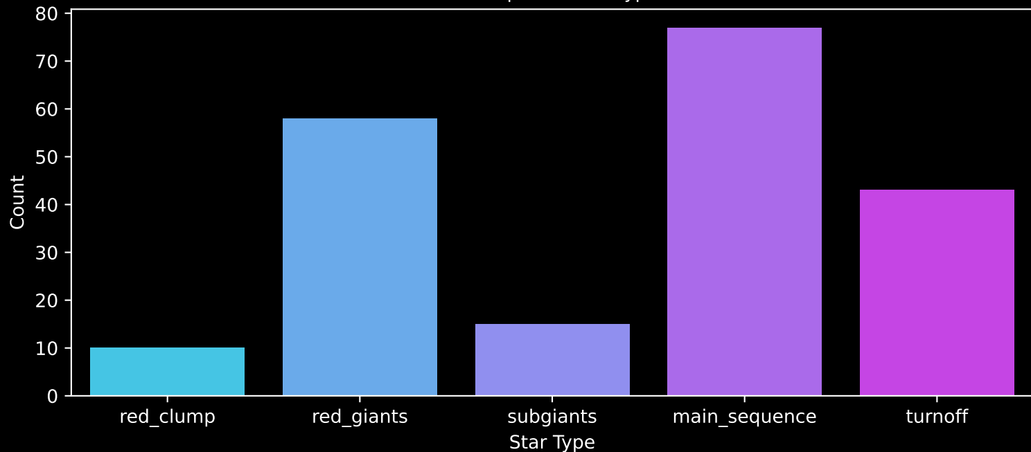
APOGEE DR17 Field: [178+26_MGA] Count plot of Star Type
