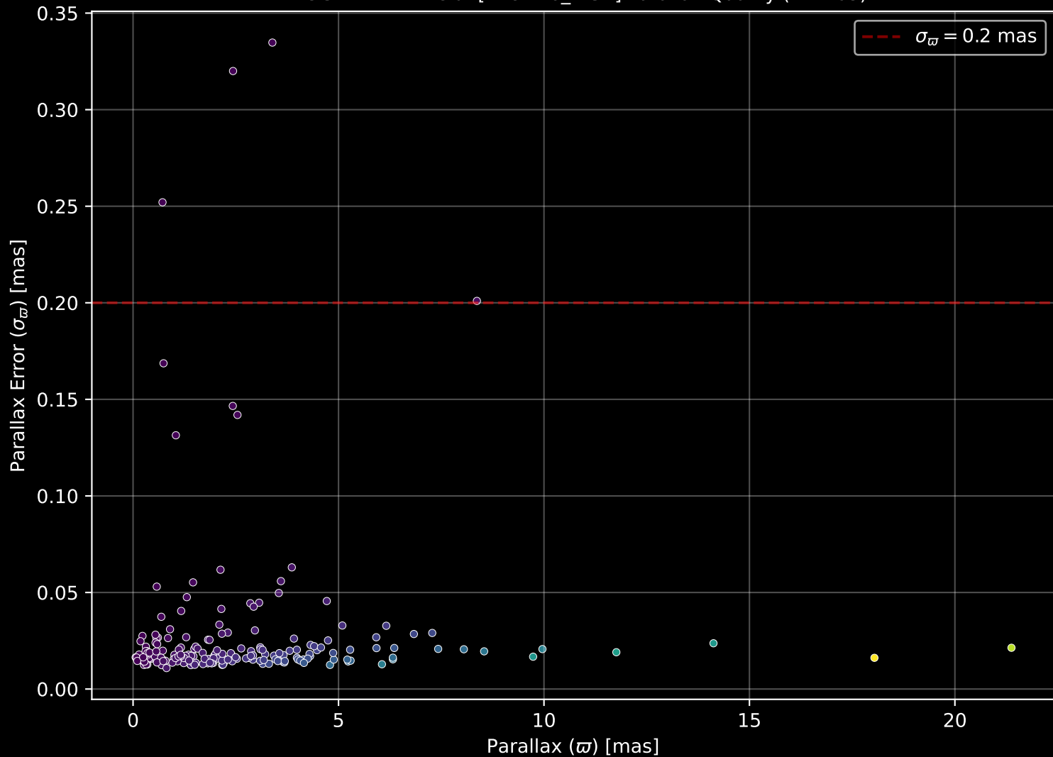
APOGEE DR17 Field: [178+26_MGA] Parallax Quality (n= 203)
