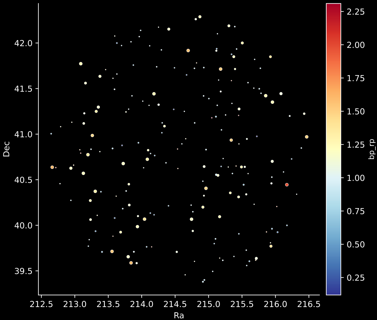
APOGEE DR17 Field: [178+26_MGA] Stars: 203
